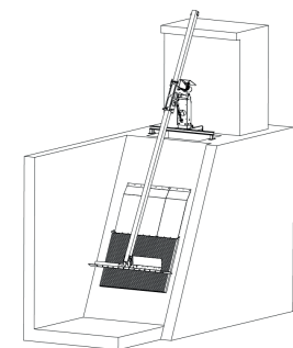
Power plant with Enerquip gate cleaner: - Nordkraft, Narvik
